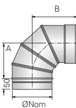
0-90° Adjustable Bend
