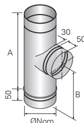
95° Tee
