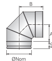
90° Fixed Bend
