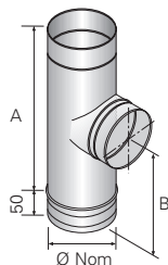
90° Tee Female Branch
