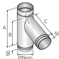
135° Tee
