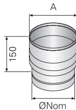
Increaser
