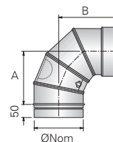
0-90° Adjustable Bend Inspection
