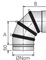
0-90° Adjustable Bend Condensing
