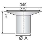
Sump Adaptor
