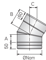
30° Bend
